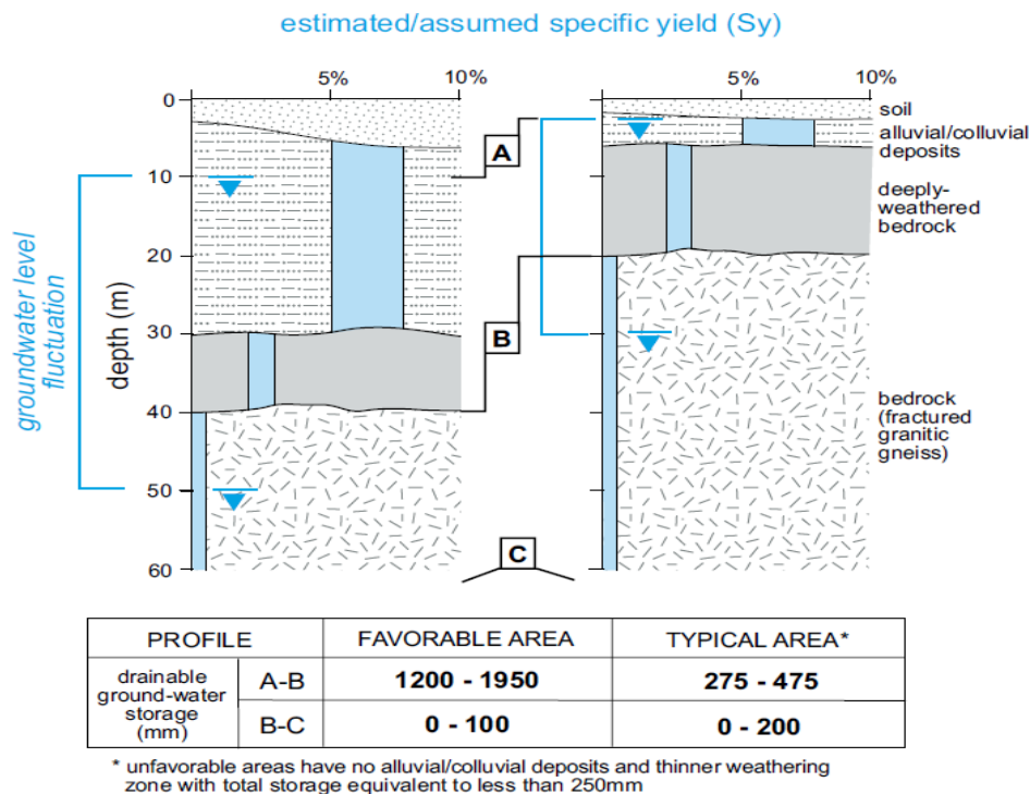
Figure 9: Typical weathered basement aquifer profiles with estimates of available groundwater storage
